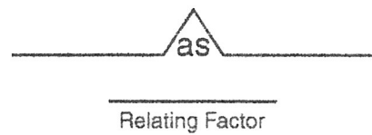
Bridge Map
