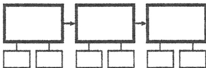
Flow Map
