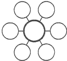
Bubble Map
