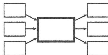
Multi-Flow Map
