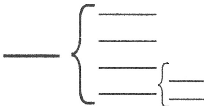
Brace Map
